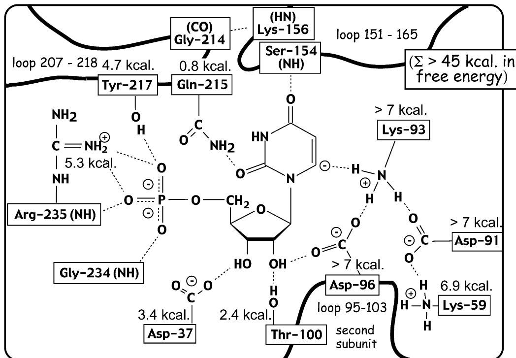
Fig. 5. Effects on the transition-state binding affinity of yeast OMP decarboxylase [59].
