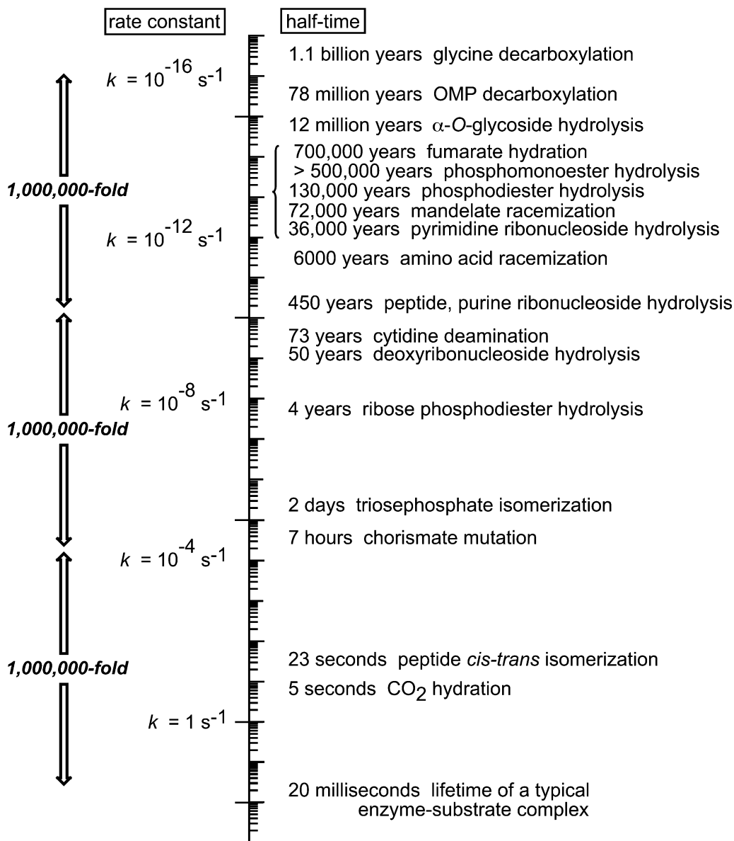
Fig. 4. Rate constants and half-times of biological reactions proceeding spontaneously in water in the absence of enzymes.
