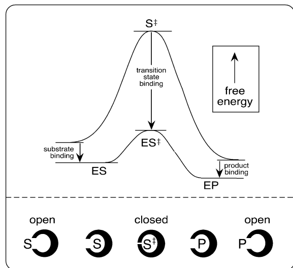
Fig. 2. A role for conformation changes in enzyme catalysis. An open configuration of the enzyme permits diffusion-controlled access of substrate and egress of product. A closed configuration of the enzyme allows maximal contact between the enzyme and substrate in the transition state.
