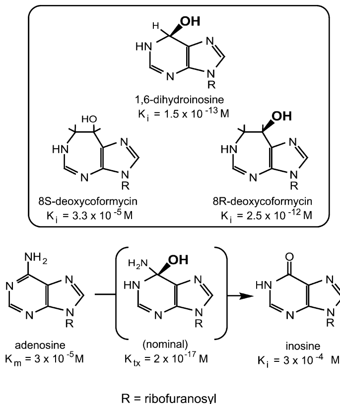
Fig. 1. Dissociation constants of ligands from calf intestinal adenosine deaminase.
