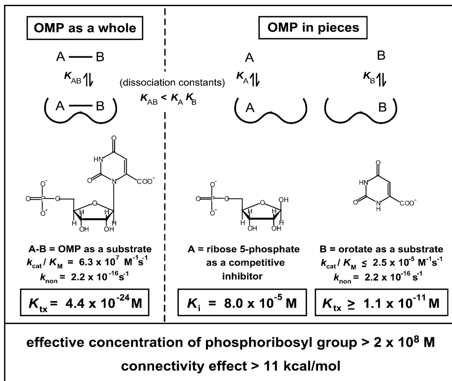
Fig. 3. Comparison of the binding affinity of yeast OMP decarboxylase for OMP, in the transition state for its decarboxylation, with orotic acid in the transition state for its decarboxylation, and for ribose 5-phosphate, the 'missing piece', as a competitive inhibitor. The effective concentration of the substrate in the transition state, > 10^8 \text{ M} , expresses the advantage the substrate gains by having its parts properly connected.
